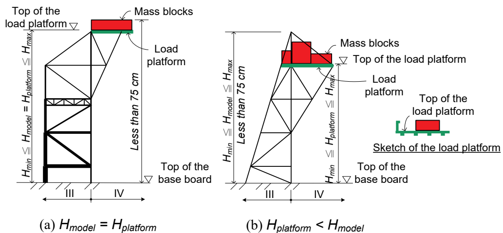
Figure 3. Sketch of the elevations of models
