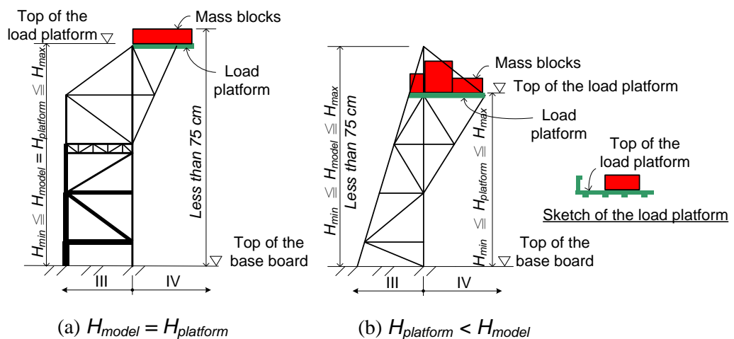
Figure 2. Sketch of the elevation of a model
