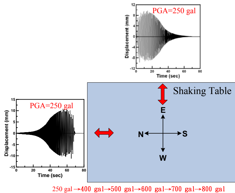
Figure 12. The input displacement time histories in the EW and NS directions.
