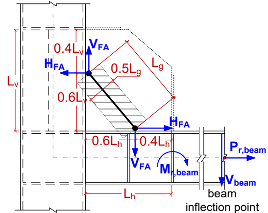
Figure 5 The equivalent strut model for computing force distributions of frame action effect.
