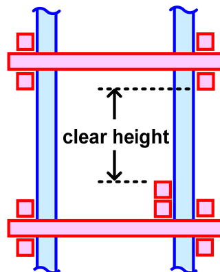
Figure 5. The definition of a clear floor height (side view)
