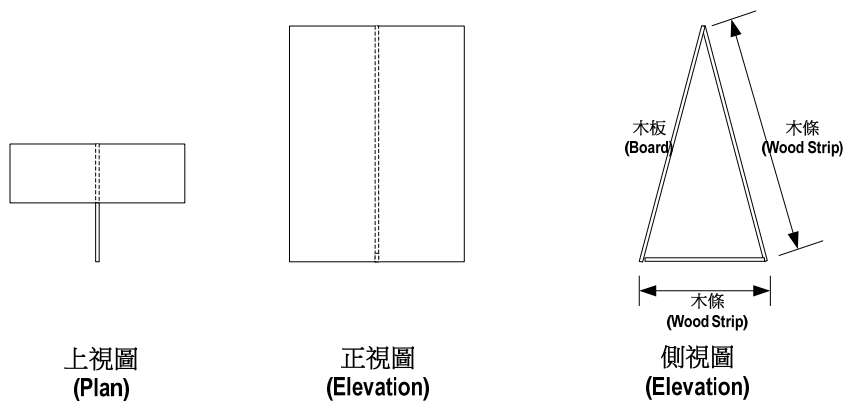
Figure 17. The poster exhibition frame.
